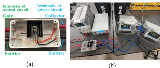
Fig 4. Terminals of control circuit and power circuit of the IGBT under analysis (a) and measurement circuit (b).
